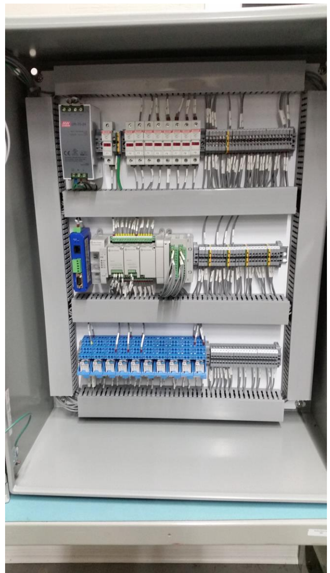
Sluice gate control cabinet interior
